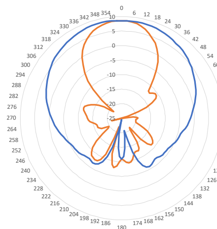
Azimuth (Blue) and Elevation (Orange) Pattern for Vertical Polarized Element
