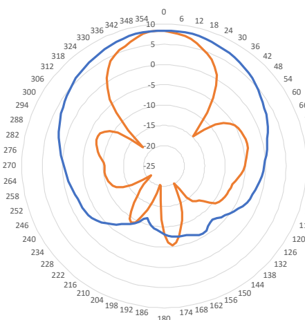
Azimuth (Blue) and Elevation (Orange) Pattern for Slant Left Polarized Element
