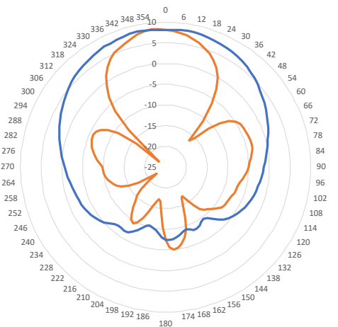
Azimuth (Blue) and Elevation (Orange) Pattern for Slant Right Polarized Element
