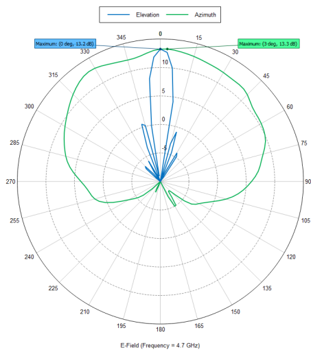
Azimuth (Green) and Elevation (Blue) Pattern for Vertical Polarized Element
